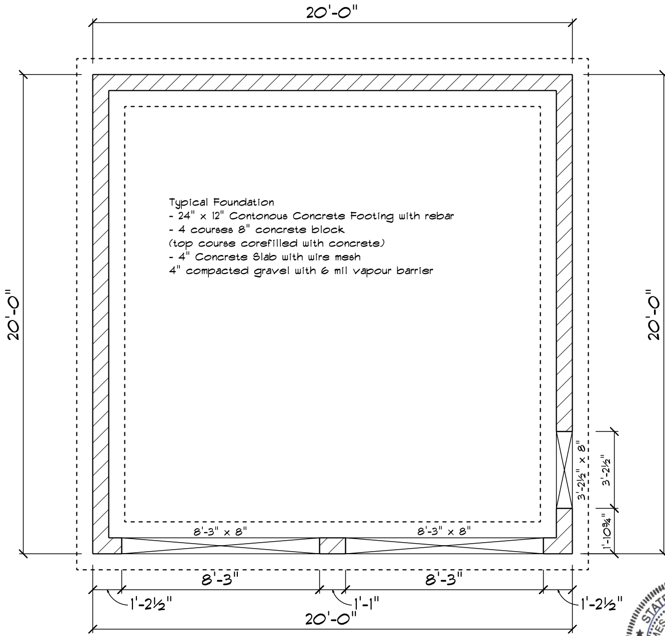
Foundation Plan
