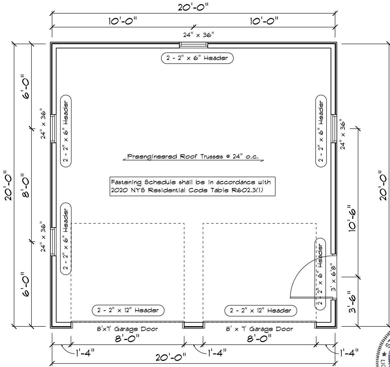
Floor Plan
